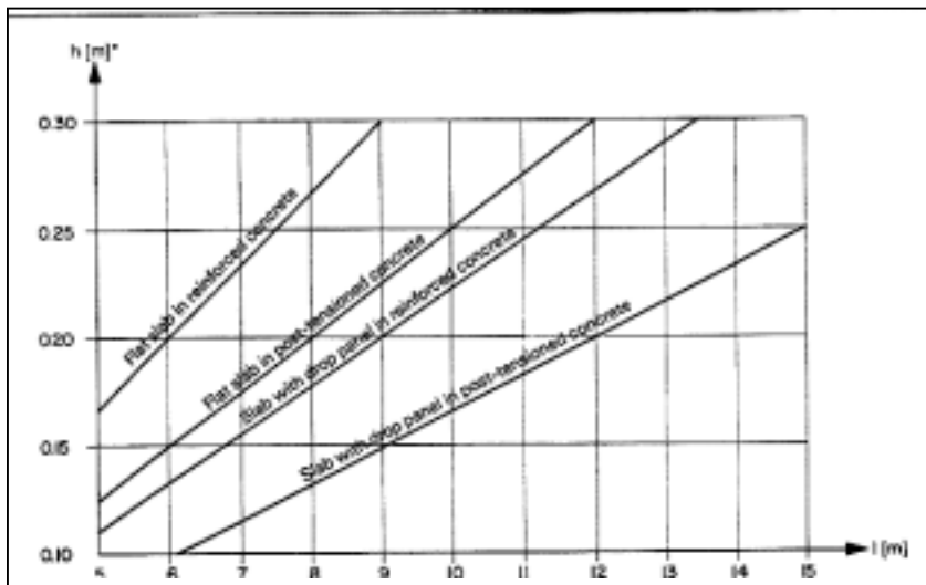
Figure 2: Slab thicknesses as a function of span lengths (recommended limits slendernesses)
