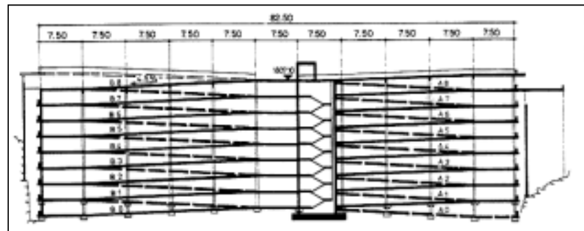
Figure 105: Longitudinal section
