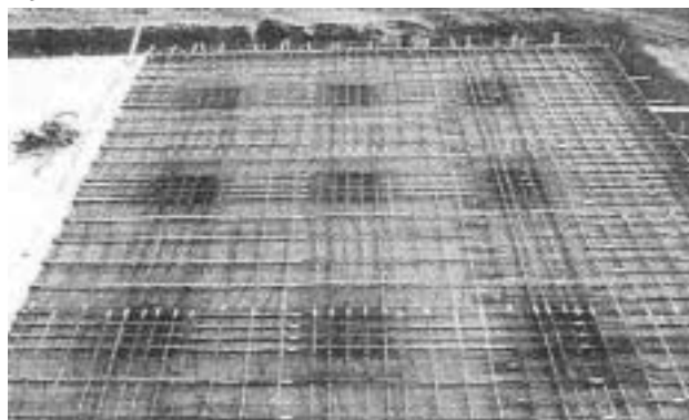
Figure 100: Installed cables of the third section
