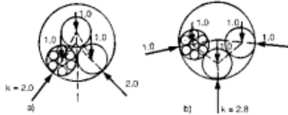
Examples of geometric position of 3 @ 0.6" strands inside a duct
