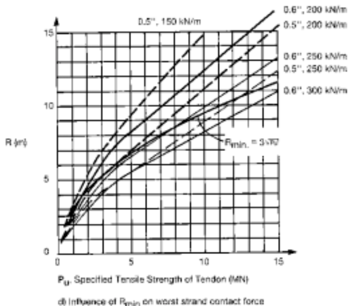
d) Influence of R_{min} on worst strand contact force
