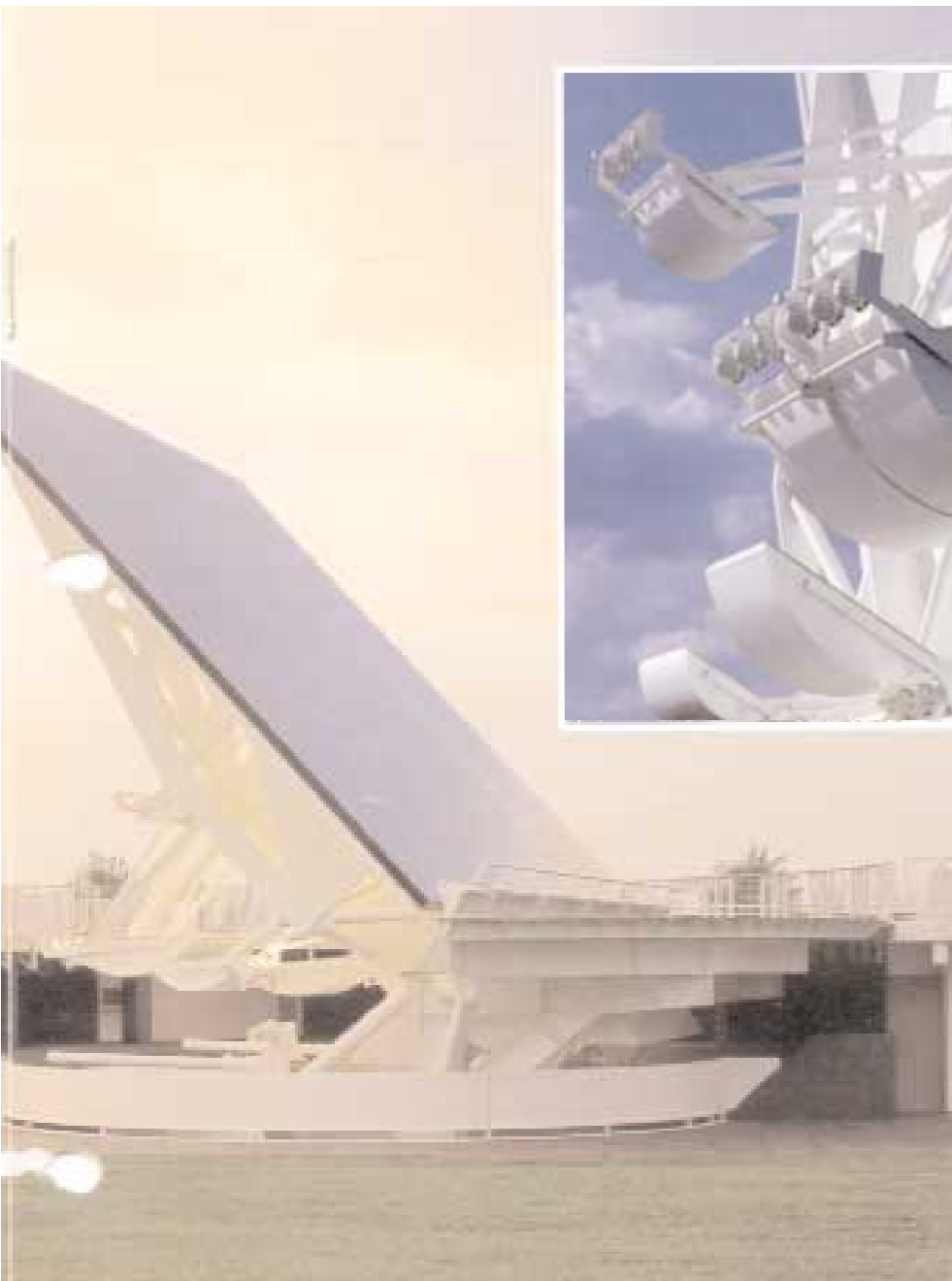
Mirrors attached to steel trusses at the rear of the rotating wall track the sun and reflect its light through the cut out names in the wall's granite.
